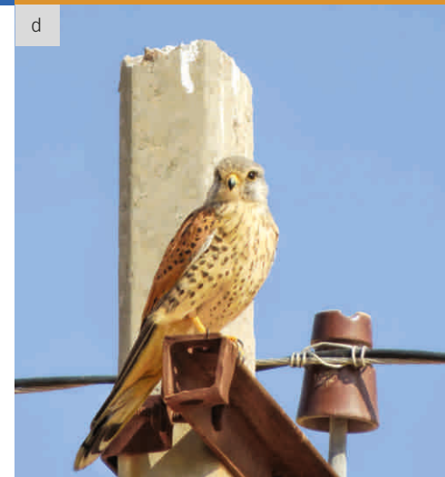
Figure 4.11. Powerlines and power poles are commonly used by birds of prey like (a) black-shouldered kite (b) buzzard (c) shikra (d) common kestrel (e) short-toed snake eagle and (f) eagle.
