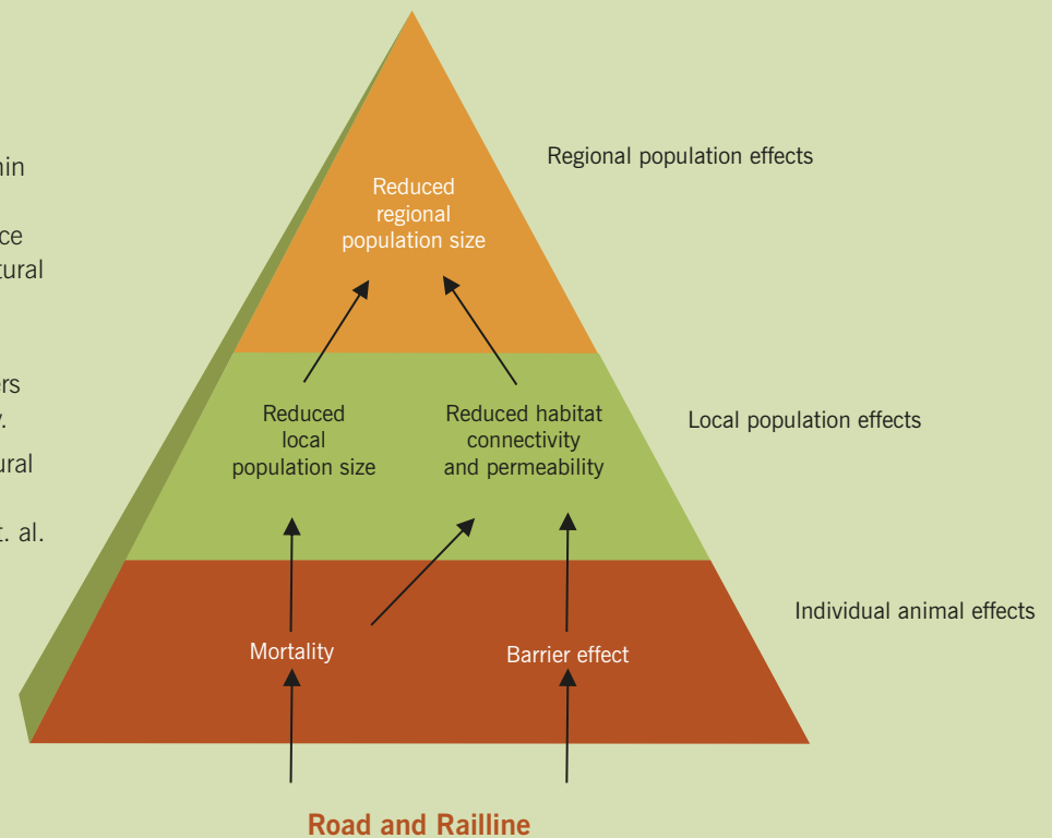
Figure 5.1. Effects of roads and rail tracks on individual animals and wildlife populations.
